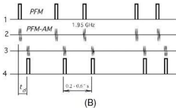
Figure (6.22): Block diagram of micropower radar (A) and the timing diagram (B).
