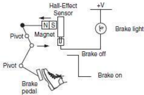
a. Hall-effect position sensor (switch)
