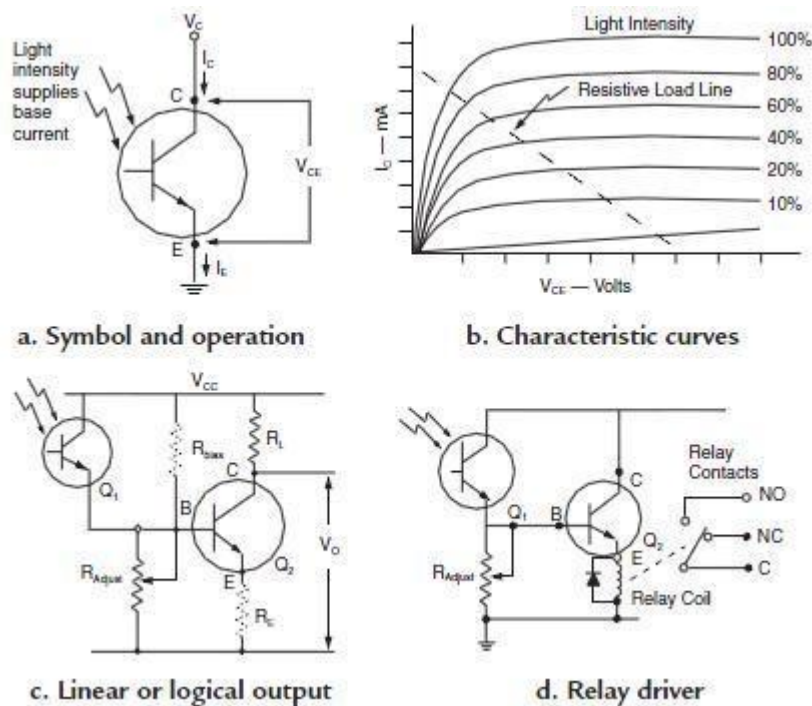
Figure (5.4): Phototransistor light sensor
