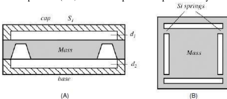
Figure (7.1): Capacitive accelerometer with a differential capacitor: (A) side cross-sectional view; (B) top view of a seismic mass supported by four silicon springs.
