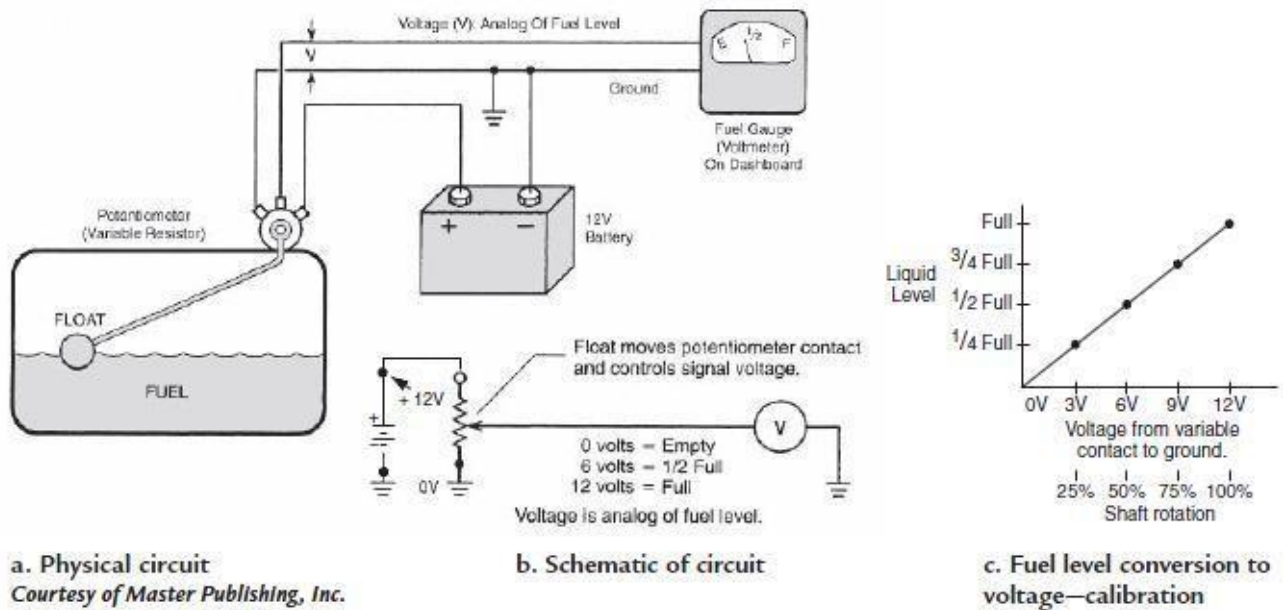
Figure (6.16): Position sensor – fuel level gauge
