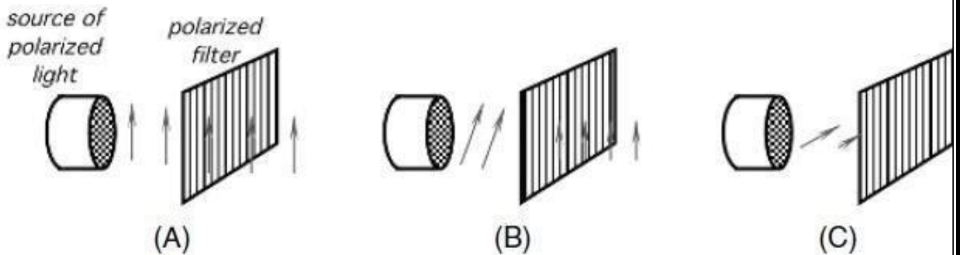
Figure (6.17): Passing polarized light through a polarizing filter: (A) direction of polarization is the same as of the filter; (B) direction of polarization is rotated with respect to the filter; (C) direction of polarization is perpendicular with respect to the filter.
