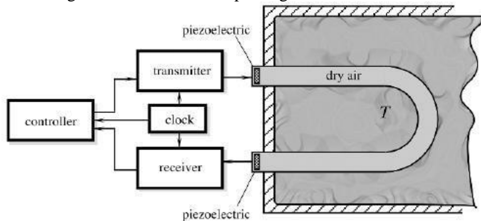
Figure (2.10): An acoustic thermometer with an ultrasonic detection system.
