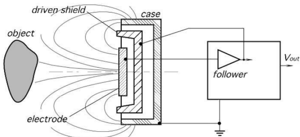
Figure (6.7): Driven shield around the electrode in a capacitive proximity sensor.
