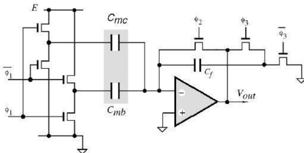
Figure (7.2): Circuit diagram of a capacitance-to-voltage conversion suitable for an integration on silicon.
