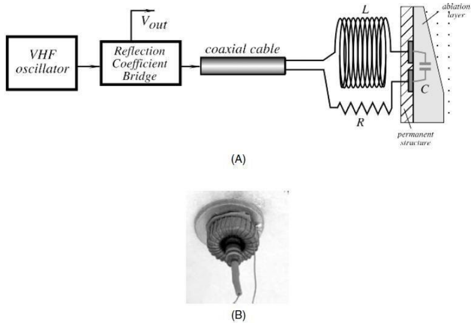
Figure (6.25): Block diagram of resonant ablation gauge (A) and prototype sensor (B).
