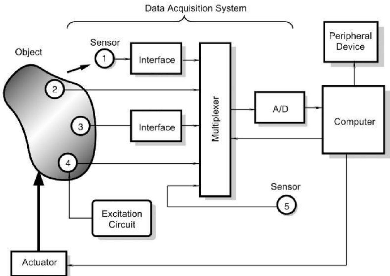
Figure (1.2): Positions of sensors in a data acquisition system. Sensor 1 is noncontact, sensors 2 and 3 are passive, sensor 4 is active, and sensor 5 is internal to a data acquisition system.
