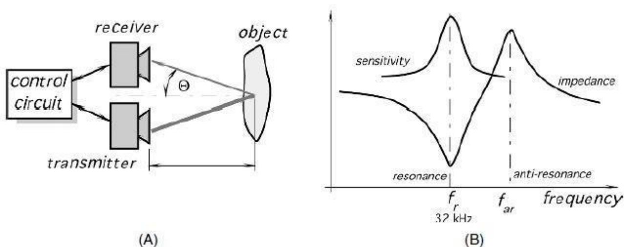
Figure (6.19): Ultrasonic distance measurement: (A) basic arrangement; (B) impedance characteristic of a piezoelectric transducer.
